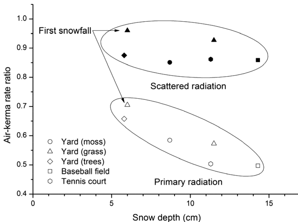
Fig. 10. Air-kerma rate reductions due to snow cover for primary and scattered radiation from deposited radiocesium. Data were obtained in first and second snowfall events.
