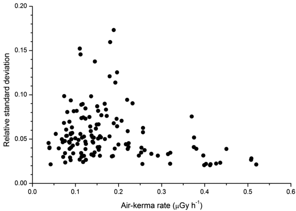
Fig. 6. Scatter plots of relative standard deviation against air-kerma rate.
