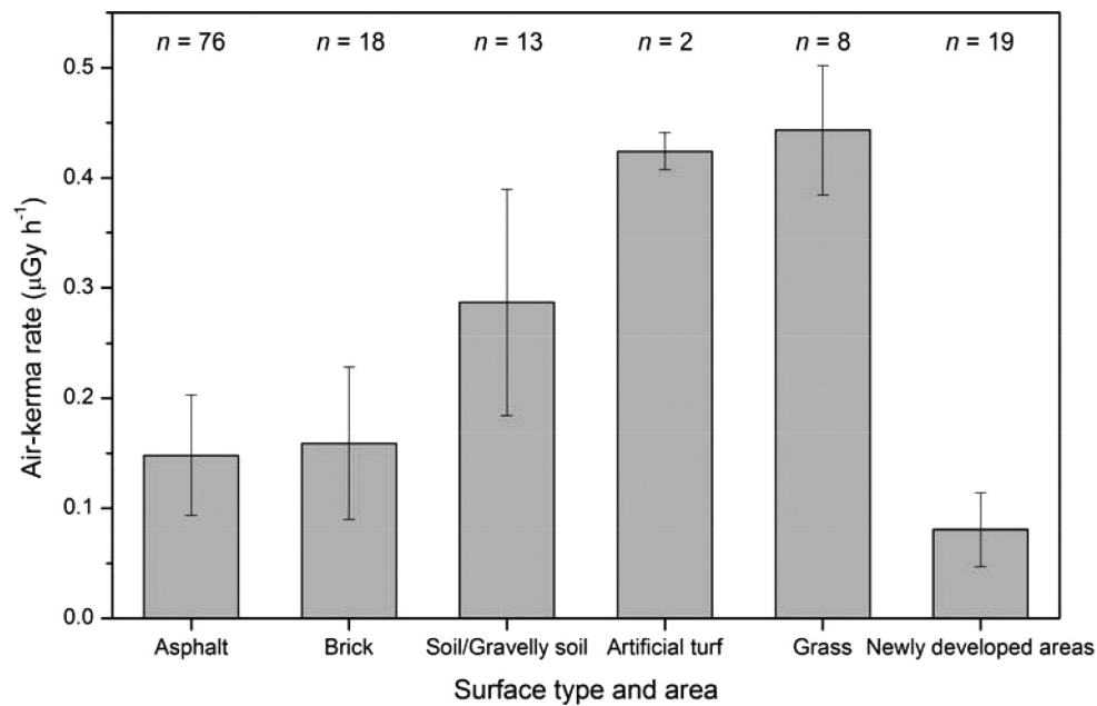
Fig. 7. Air-kerma rates on different surface types and in newly developed areas. Vertical bars represent standard errors.
