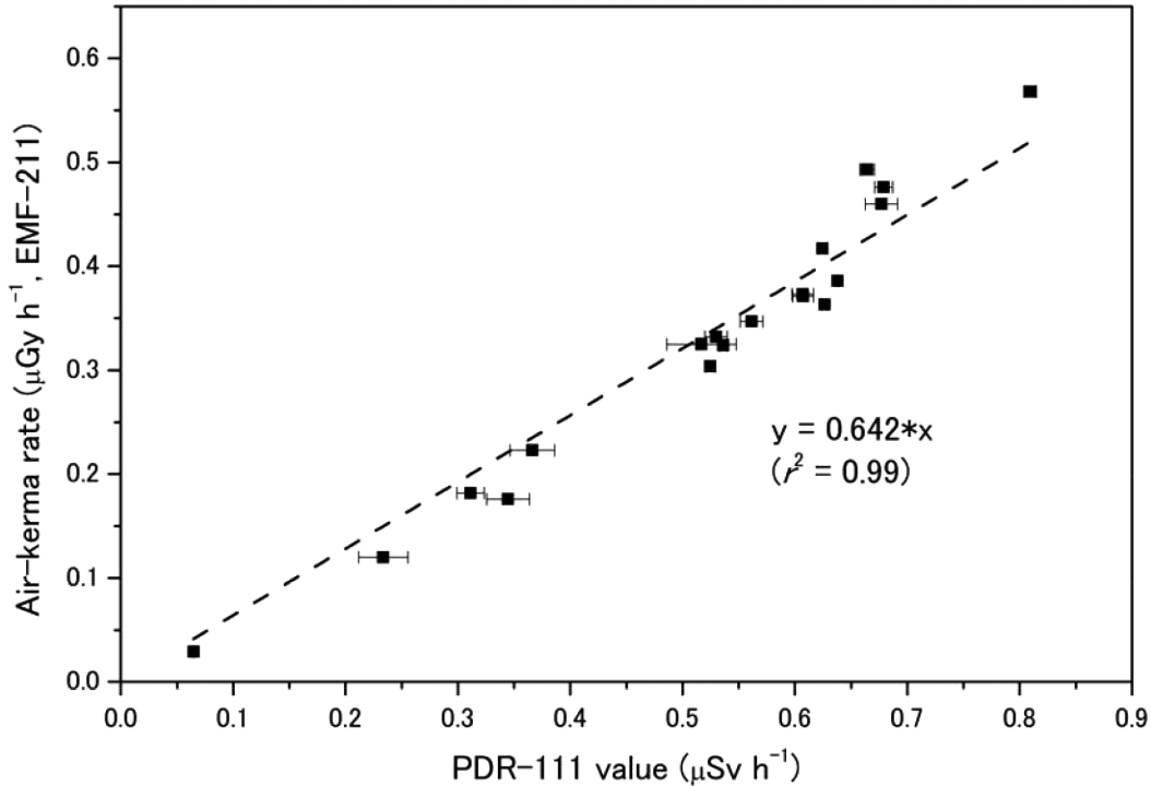
Fig. 3. Scatter plots of air-kerma rates against measured PDR-111 values. Data were obtained in presence ( n = 13 ) and absence ( n = 6 ) of snow cover. Bars represent standard deviations calculated from four measurements at each point. Broken line was fitted assuming intercept of zero.
