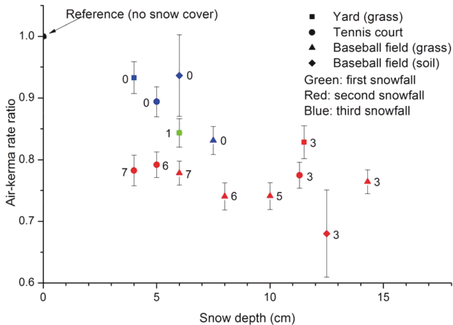
Fig. 9. Scatter plots of air-kerma rate ratio in presence and absence of snow cover. Ratio is unity with no snow cover. Reference value was calculated from two air-kerma rates obtained on separate days. Vertical bars were evaluated based on error propagation. Suffix numbers represent lapsed days after snowfall.
