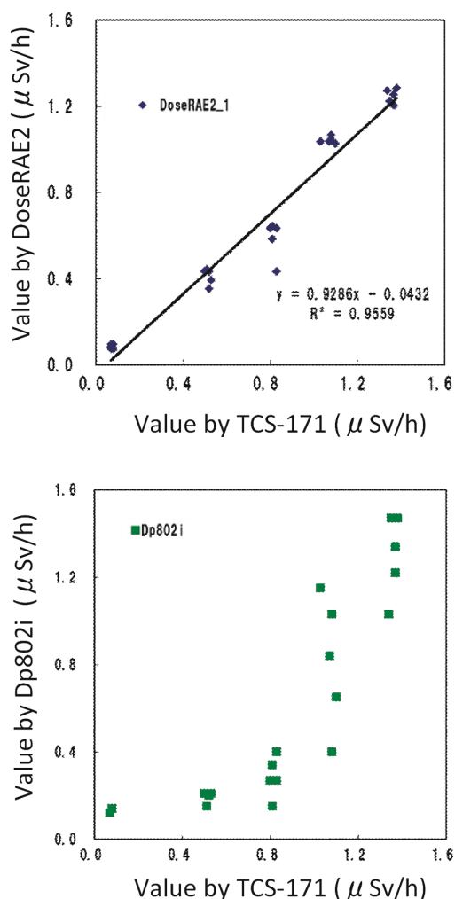
Fig. 11. Correlation of doses measured by DoseRAE2 with the CsI (Tl) scintillation, Dp802i with GM tube, and TCS-171B under the same condition.
