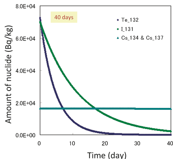
Fig. 5. Calculation of the transition of nuclide.
