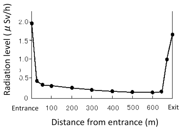
Fig. 10. Distribution of radiation level in a tunnel of about 800 m in length in Fukushima City.
