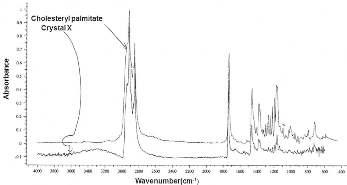
Fig. 3 – The infrared spectra of cholesterol-like crystals (Crystal X) and cholesteryl palmitate. The spectrum of Crystal X and cholesteryl palmitate is identical.
